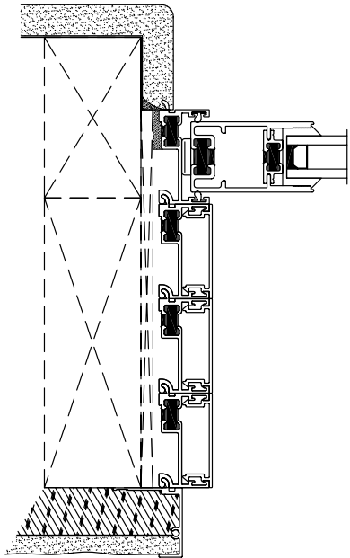
Deep Wall Install 2x6 and 2x4 ▶ 1.375" Stucco Return
